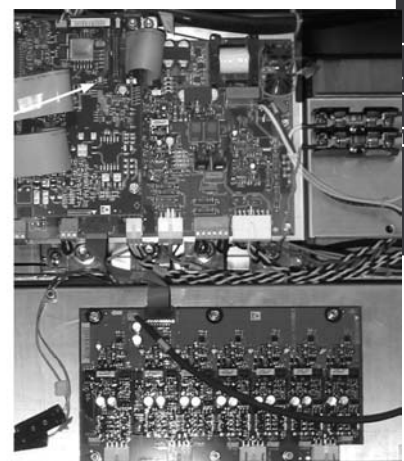
Compact IP 54 VLT 5072 - 5102 380 - 500 V
