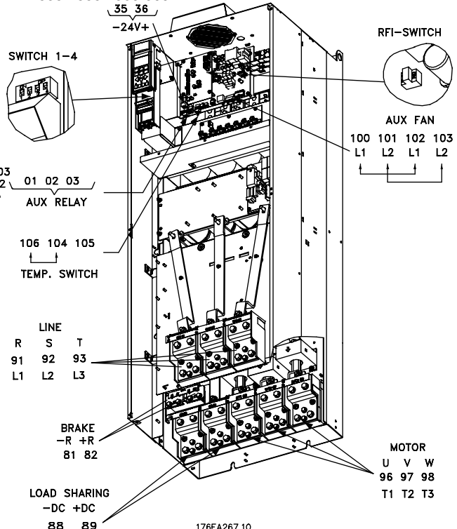
Compact IP 00 without disconnect and fuse VLT 5352-5552 380-500 V
