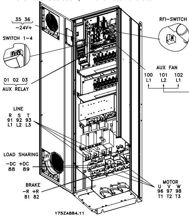
Compact IP 00 with disconnect and fuse VLT 5202-5302 380-500 V, VLT 5202-5352 525-690 V
