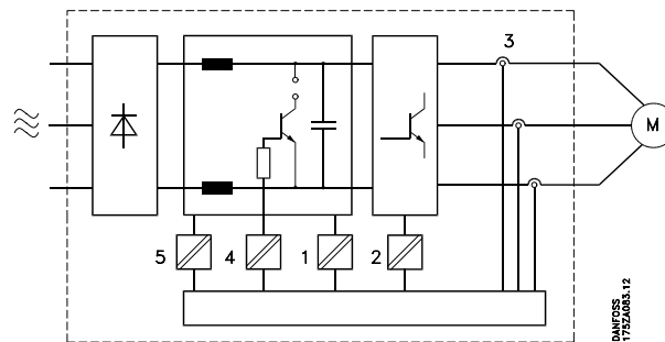
Galvanic isolation
