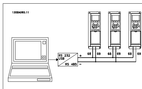
Illustration 5.6: Exemple de raccordement.
