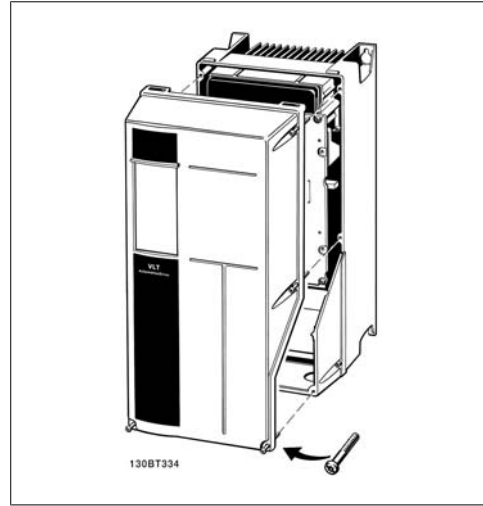
Illustration 4.17: A5, B1, B2, C1 ve C2 muhafazalar
