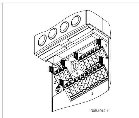
Illustration 4.18: Bornes de commande (toutes protections)
