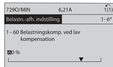
Illustration 7.11: Displayeksempel.
