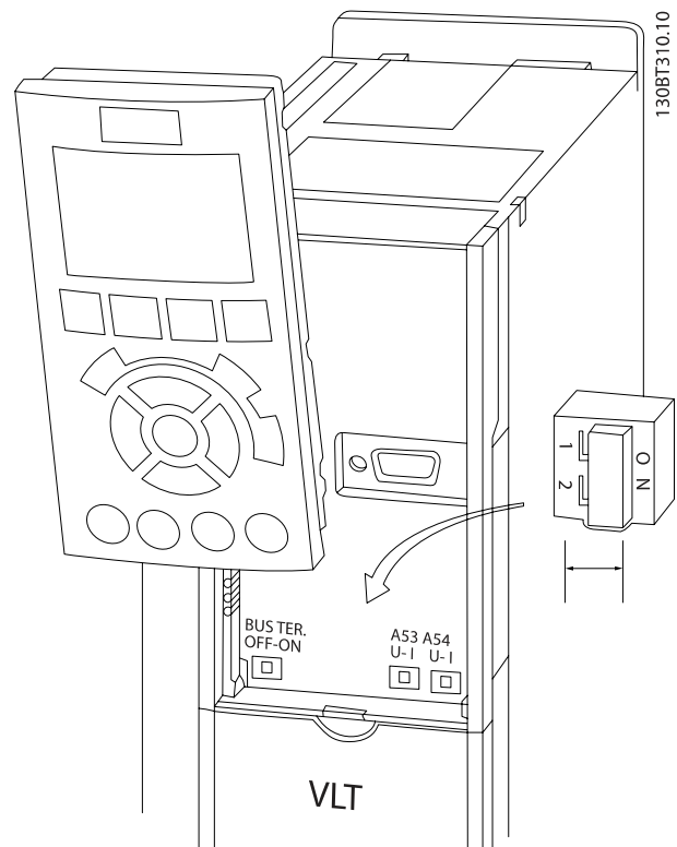
Illustration 4.44: Kontaktplacering.
