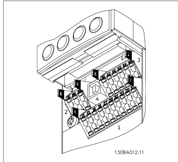
Illustration 5.31: Styreklemmer (alle kapslinger)
