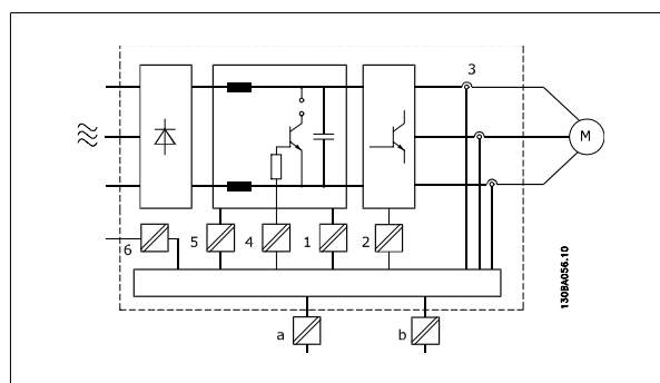
Illustration 2.6: Galvanisk adskillelse
