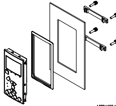
Figure 3.6: LCP kit with numerical LCP, fasteners and gasket.
