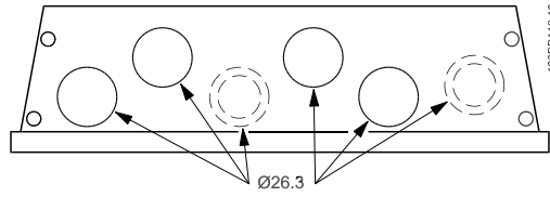
Figure 5.9: Cable entry holes for enclosure A5. The suggested use of the holes are purely recommendations and other solutions are possible.
