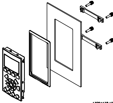
Figure 3.5: LCP kit with graphical LCP, fasteners, 9.8 ft [3 m] cable and gasket.
