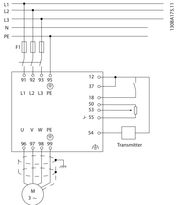
Illustration 3.7 Two-wire transmitter
