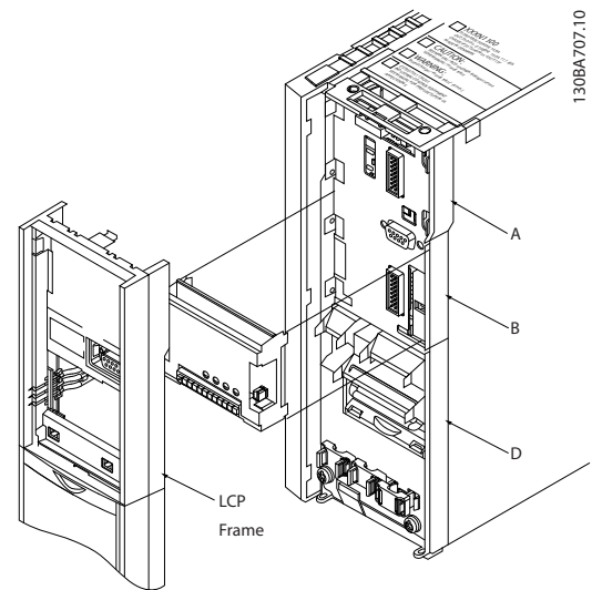
Illustration 10.1 Frame sizes A2, A3 and B3
