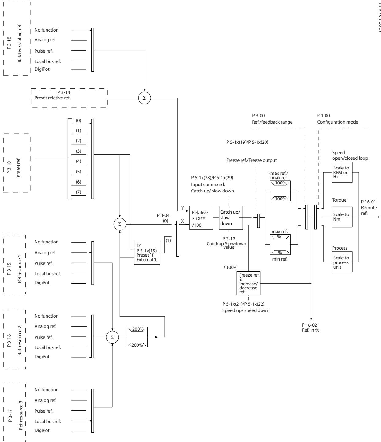
Illustration 3.3 Remote reference
