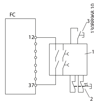
Illustration 3.18 STO example
