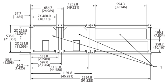
Illustration 7.50 Frame Size F4
