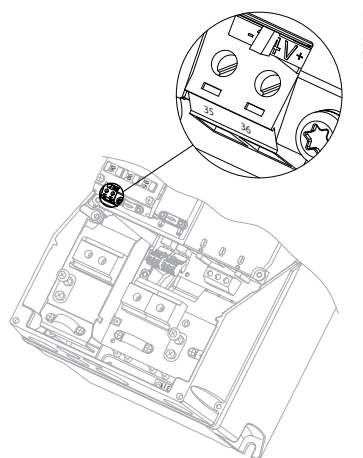
Illustration 10.8 Connection to 24V back-up supply on frame sizes A5, B1, B2, C1 and C2.
