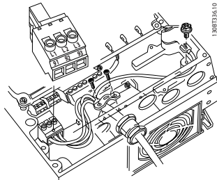
Mains connector frame size A4/A5 (IP 55/66)
