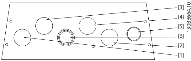
Illustration 8.18 A5 - IP55
