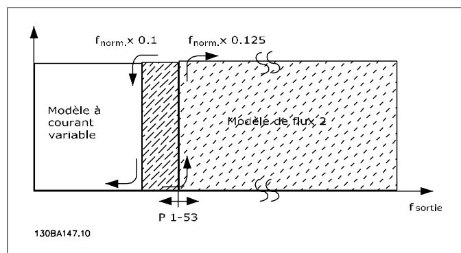
Illustration 2.3: Par. 1-00 = [0] Boucle ouverte vit. Par. 1-01 = [2] Flux ss retour
