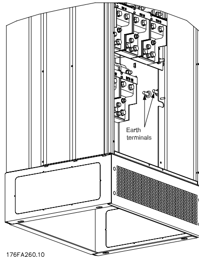
176FA260.10 Position of earth terminals, IP 21/ IP 54
