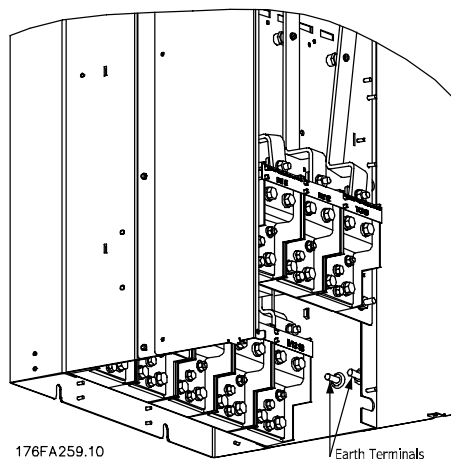
Jordplintarnas position, IP 00
