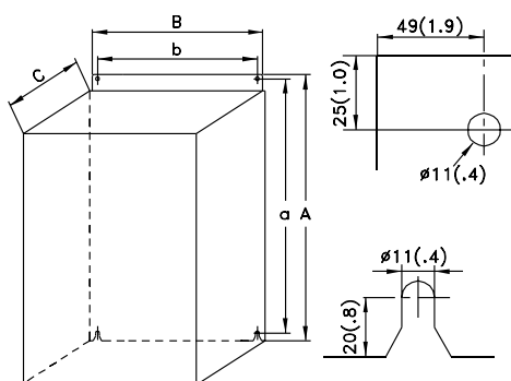
Modell I, IP 00
