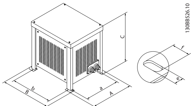
Illustration 5.14 IP23 Floor Mounted
