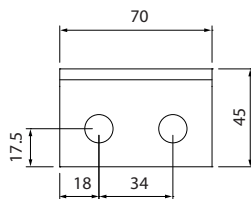
Illustration 5.16 L-shaped Terminal Kit 130B3138
