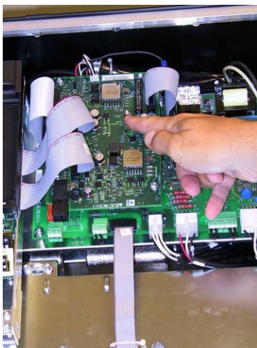
Photo 13: RFI Switch on Control Card
