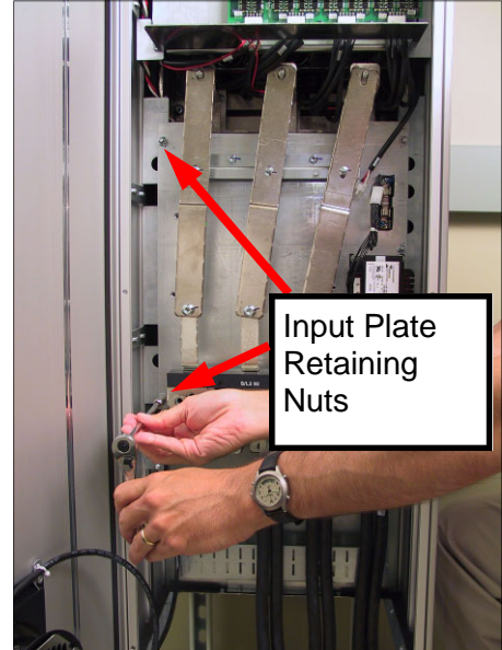
Photo 5. Removing Input Plate Retaining Nuts
