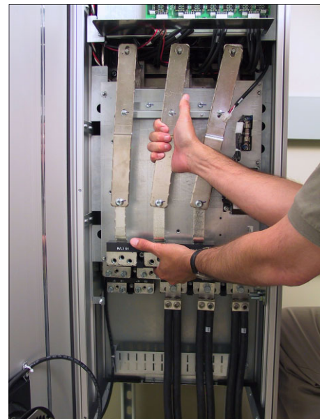
Photo 6. Removing Input Plate
