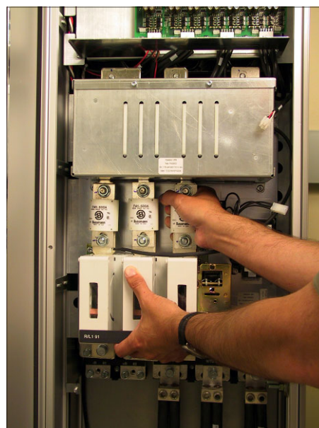
Photo 10. Installing Input Plate with Disconnect, Fuses and RFI
