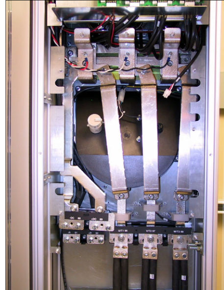
Photo 7. VLT Frame D2 with Input plate removed
