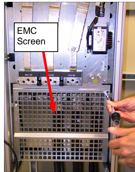
Photo 2. Input Power cables removed
