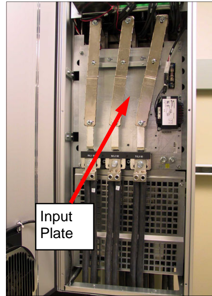
Photo 1. Frame D2 VLT without options
