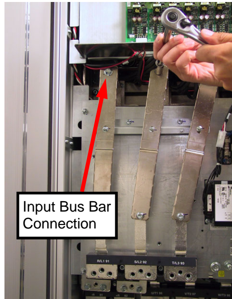
Photo 3. Input Plate Bus-Bars
