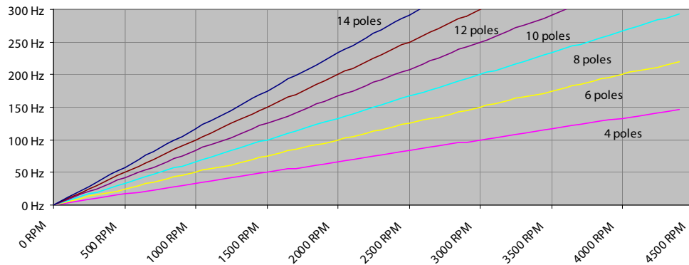
Relation between actual motor frequency, number of poles and resulting speed (50 Hz oriented)
