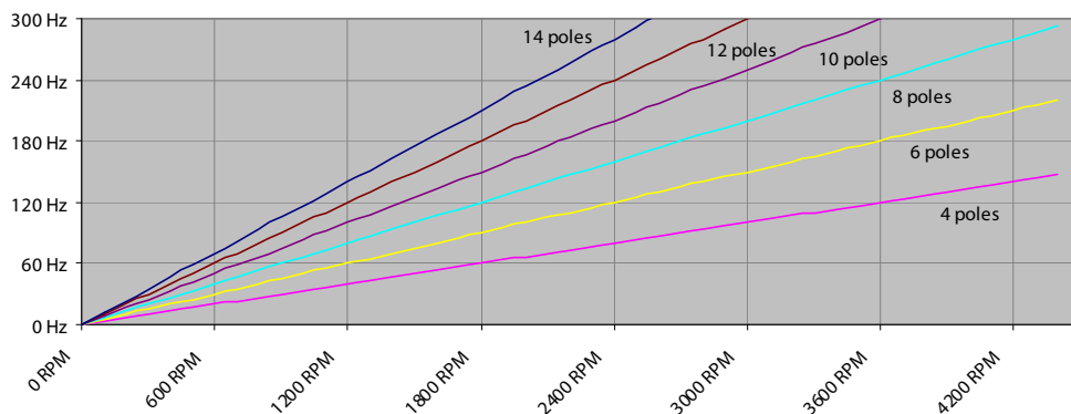
Relation between actual motor frequency, number of poles and resulting speed (60 Hz oriented)
