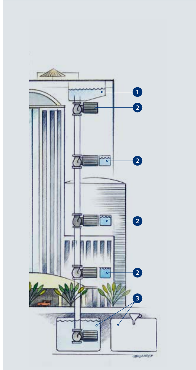
Traditional sprinkler
